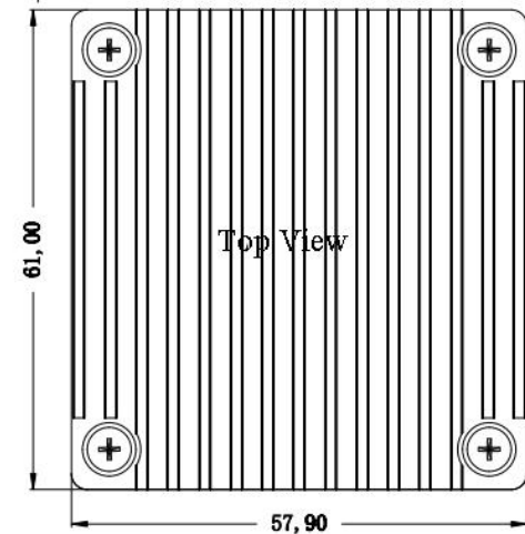
Standard+Heatsink 61*57.9*27.7mm
