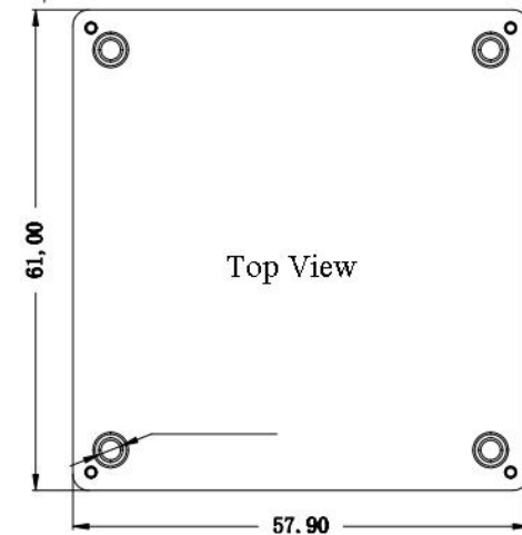
Standard 61*57.9*12.7mm
